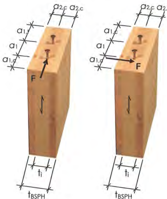
Figure 6: Definitions of minimum spacings, edge and end distances for laterally loaded dowel-type fasteners in the narrow side of cross laminated timber
